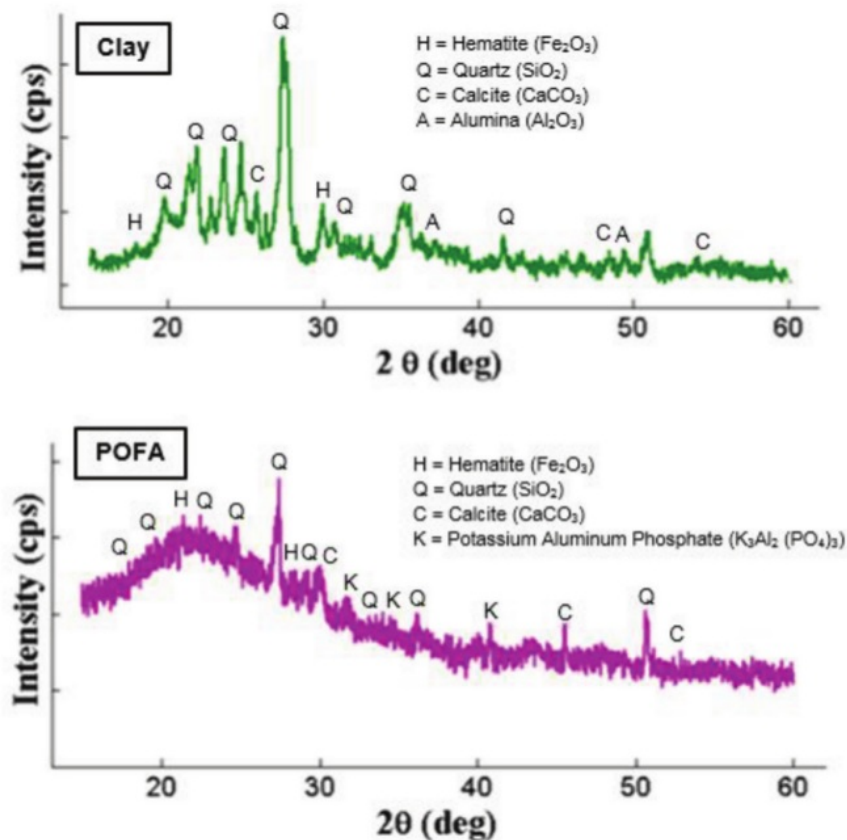
15 Figure 1. XRD patterns of the clay and POFA used to manufacture bricks.
