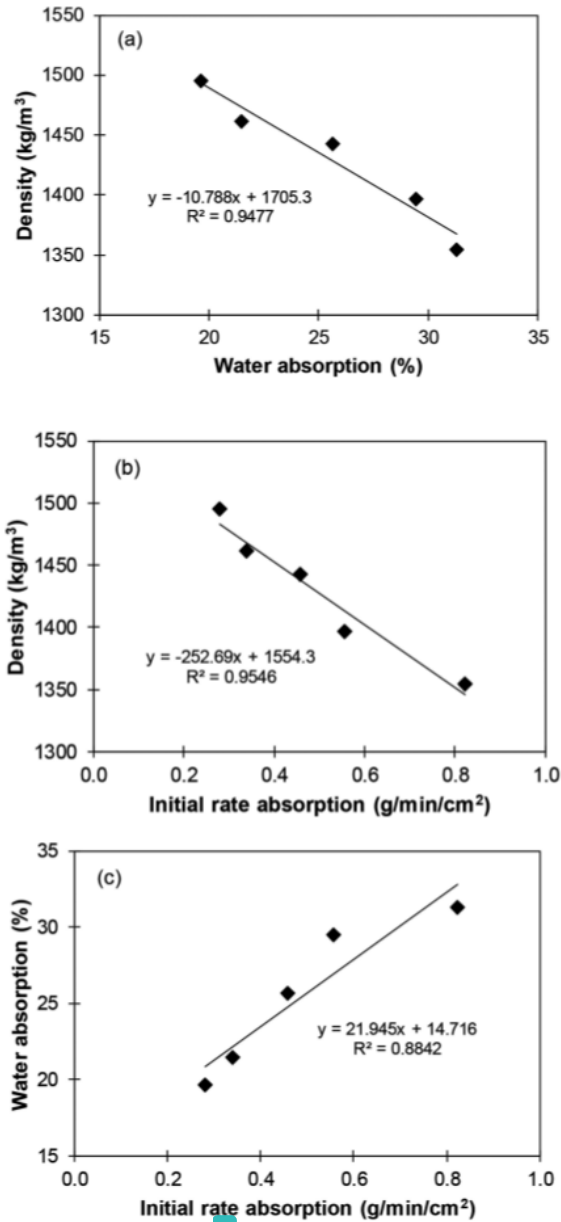
Figure 13. Linear relationship between pairs of physical properties: (a) density and water absorption; (b) density and initial rate absorption; (c) water absorption and initial rate absorption.
