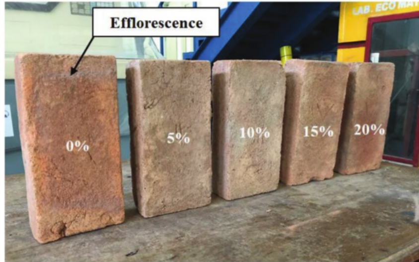
Figure 9. Efflorescence of brick specimens with different POFA contents.
