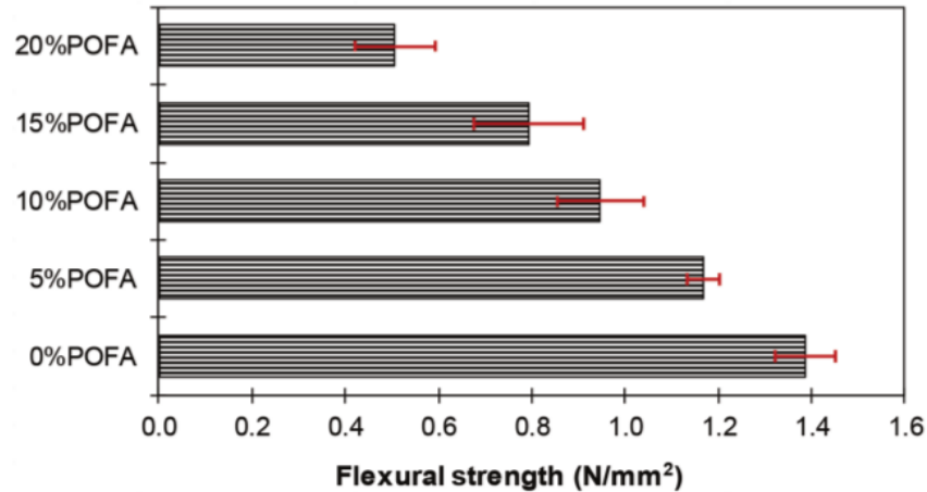
Figure 7. Flexural strength of bricks with different levels of clay replacement with POFA.
