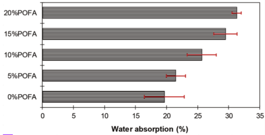
27 Figure 5. Effect of POFA on the water absorption properties of bricks.
