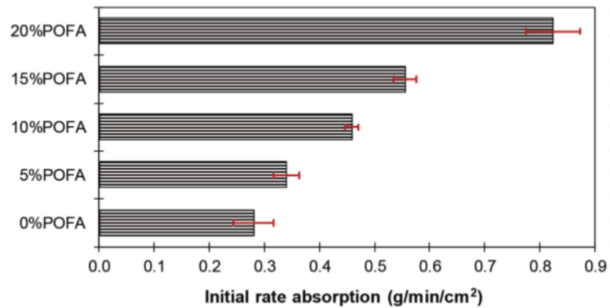
21 Figure 6. Effect of POFA on the initial rate of absorption of bricks.
